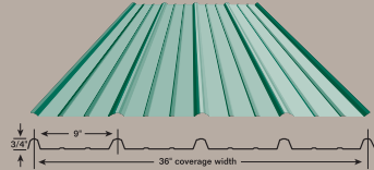
Standard Residential Panel
