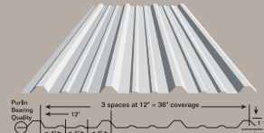
PBR Commercial / Residential Panel
