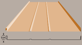
Secure-Seam Standing Seam Panel
